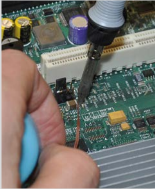
Desoldering with a solder wick
