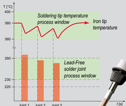
Temperature curve of controlled tip temperature when soldering multiple joints
