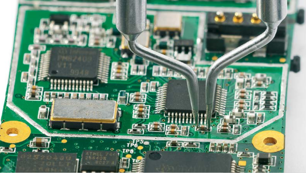
SMD desoldering in 3 seconds – with the Ersa desoldering tweezers
