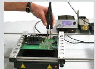
IRHP 200 infrared rework heating plate to assist in the soldering and desoldering process on multilayer boards or high-mass components
