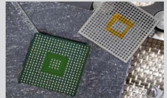
3. Reballing – adding new solder balls
