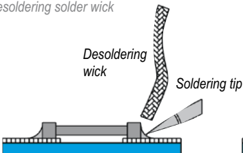
Solder melting and removal with a desoldering solder wick
